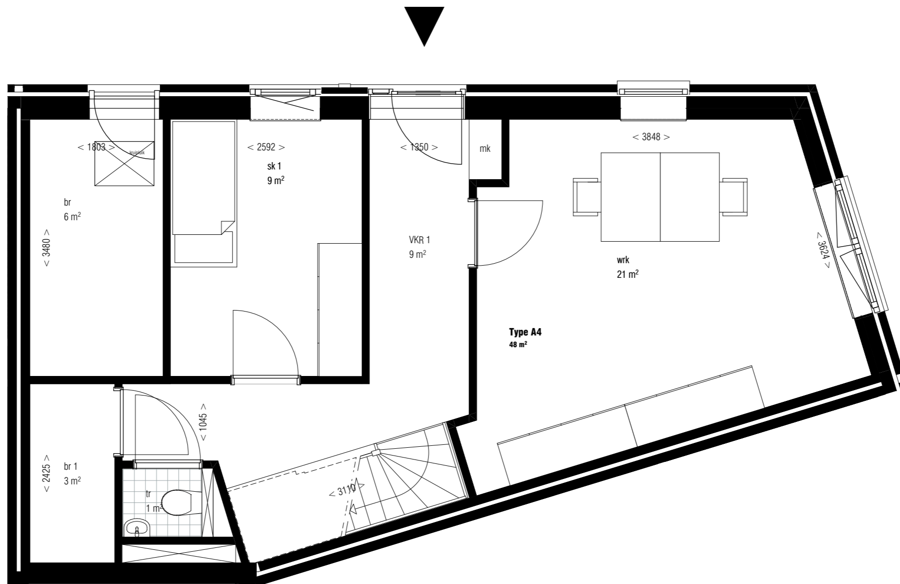
Type A4 BEGANE GROND
